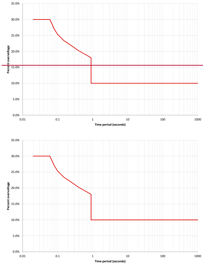
Figure 18 – Over voltage limit for contingency events
