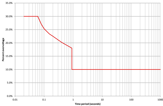
Figure 18 – Over voltage limit for contingency events
