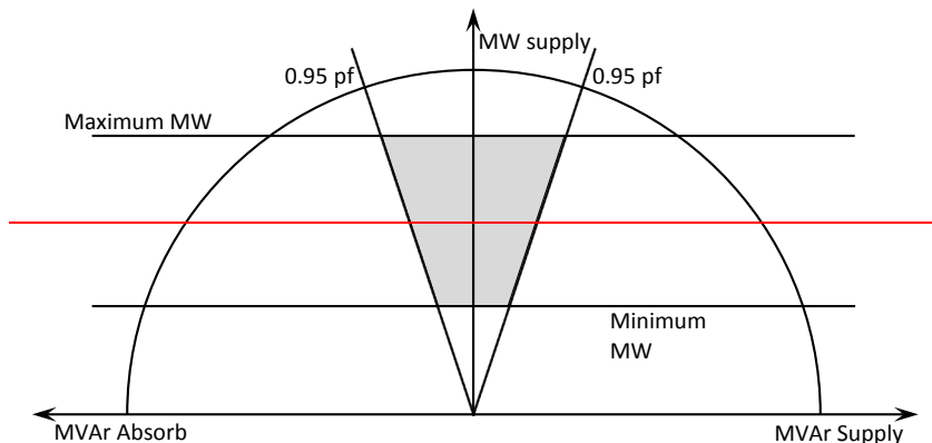
Figure 3—Inverter coupled Generation Unit reactive power capability
