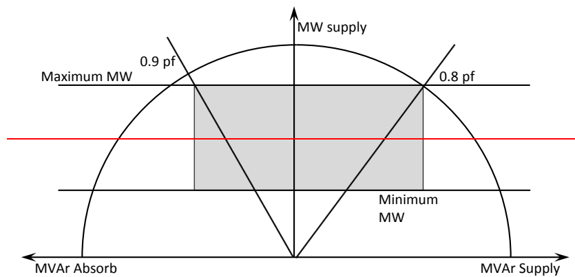
Figure 1—Synchronous Generation Unit reactive power capability
