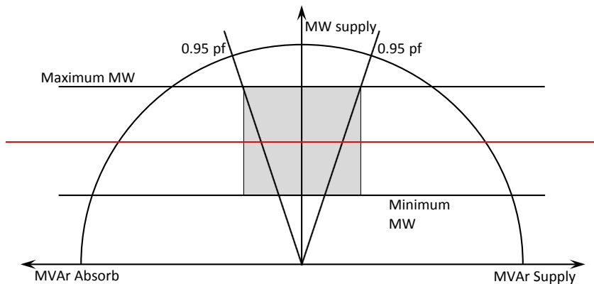
Figure 2—Induction Generation Unit reactive power capability
