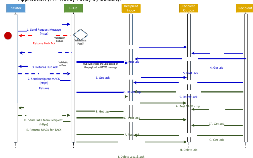
Figure 16 Interoperability – Webservices to FTP sequence diagram
