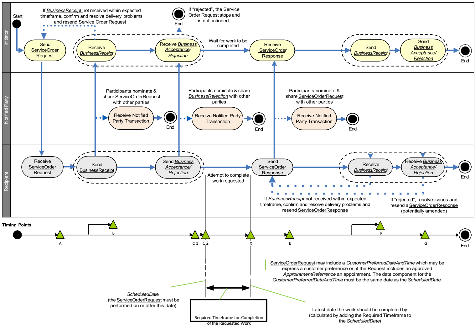
Figure 3 Timing Overview
