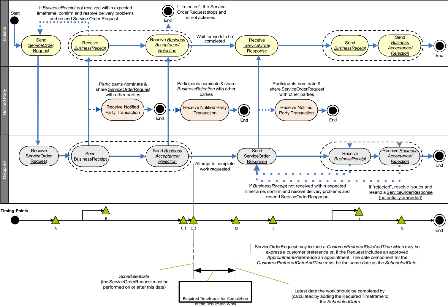
Figure 3 Timing Overview
