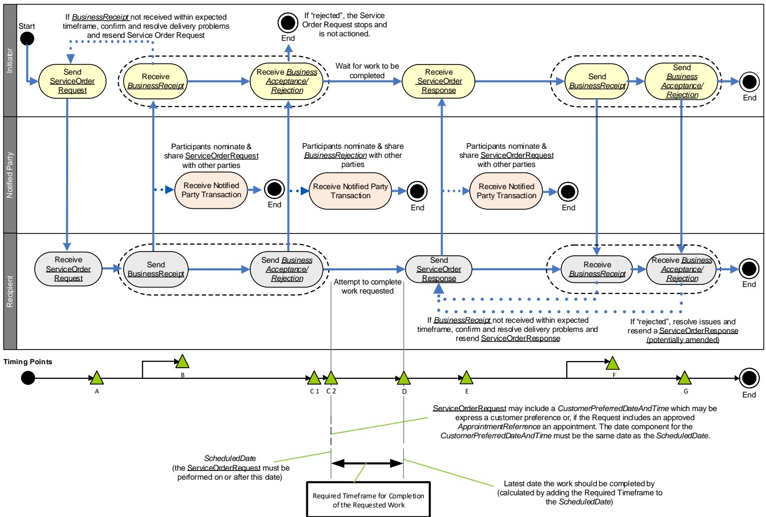
Figure 3 Timing Overview
