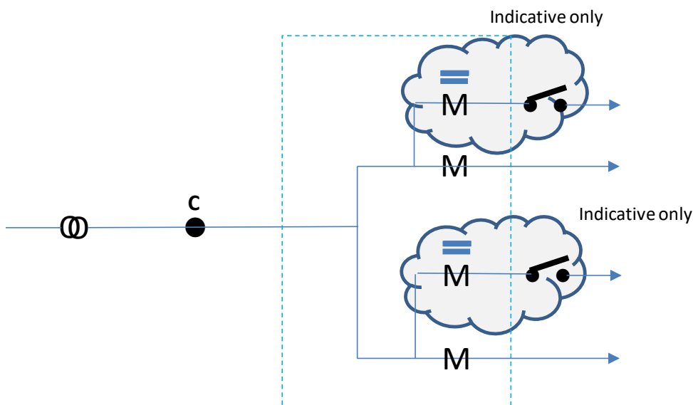
Figure 26 - One customer, two multi-function meters ( Not applicable in NT )
