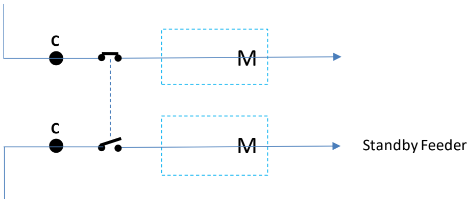
Figure 16 - One contestable customer with standby supply (eg: Robertson Barracks, Darwin Airport HV supply)
