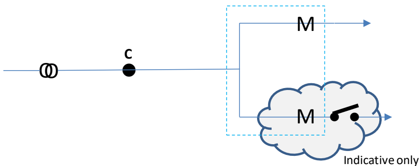
Figure 4 - Contestable customer, two tariff metering (general supply + off-peak) on the lower voltage side of the transformer
