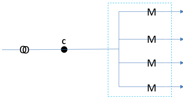
Figure 3 - Contestable customer, multiple metered on the lower voltage side of the transformer
