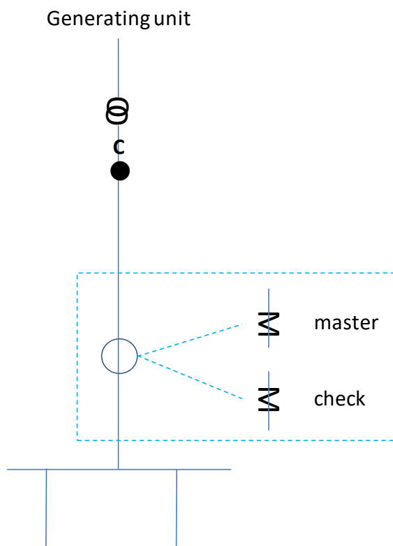
Figure 19 - Generating unit supply point at wholesale market boundary
