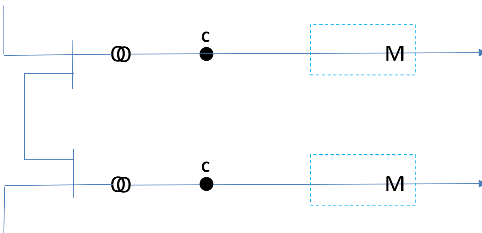
Figure 11 - One contestable customer, two separate substations adjacent to each other or one single substation with two separate transformers, with the HV supply originating from a single source and LV switchboard in common switch room. This arrangement also applies to two separate substations not adjacent to each other but on the same premise
