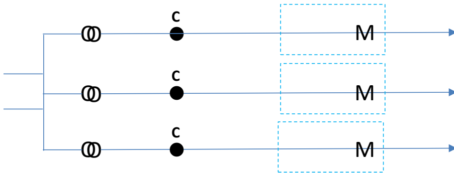
Figure 8 - Three contestable customers, metered on low voltage side of multiple transformers in the same substation building
