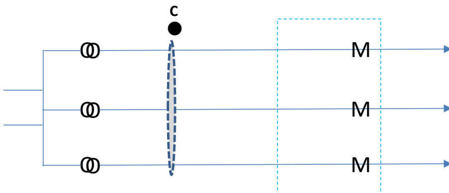
Figure 7 - Contestable customer, multiple meters on low voltage side of multiple transformers in the same substation
