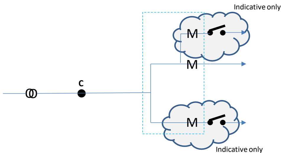
Figure 5 - Contestable customer, two controlled loads, one twin element meter
