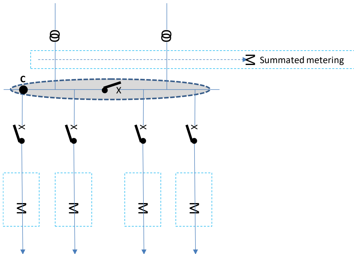
Figure 17 - Wholesale market boundary – physical metering
