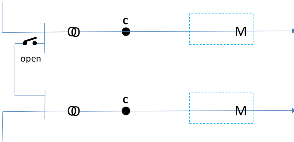
Figure 10 - One contestable customer, two separate substations adjacent to each other or one single substation with two separate transformers, with a normally open point separating the high voltage supplies into two sources
