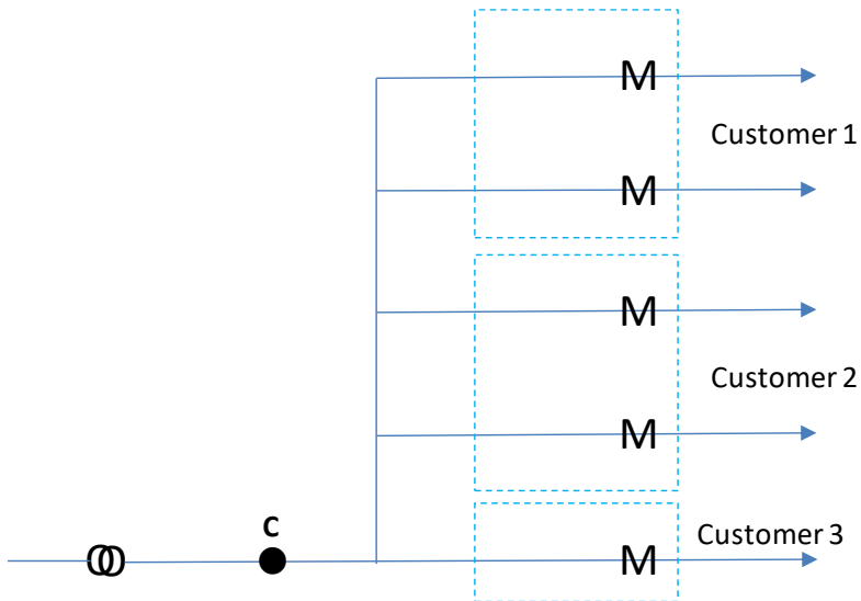
Figure 13 - Multiple contestable customers, high rise buildings
