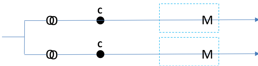
Figure 9 - Two contestable customers, two separate HV supplies to two separate substations, both metered on LV side
