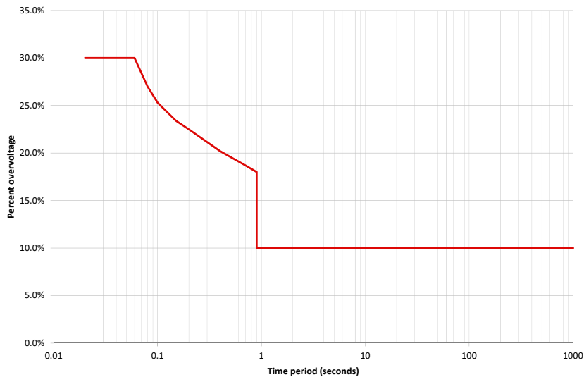
Figure 18 18 – Over voltage limit for contingency events
